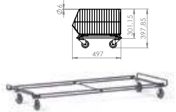
Rack Base (h x d x l) 97 x 497 x 1000 mm 97 x 497 x 1250 mm
