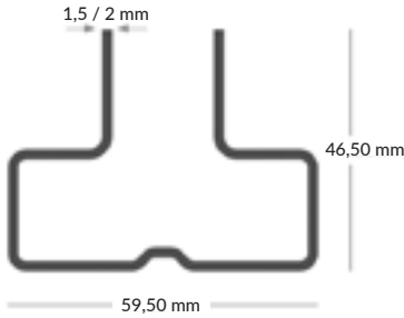
F60 MR Frame Profile Section
