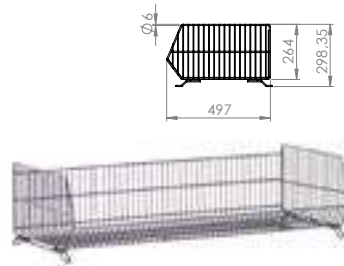
Wire Basket Rack (h x d x l) 264 x 497 x 1000 mm 264 x 497 x 1250 mm
